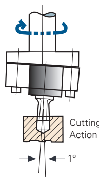
Diagram B Broaching a Stationary Work Piece
