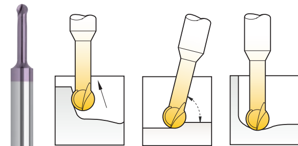
Metric Long Neck Series
