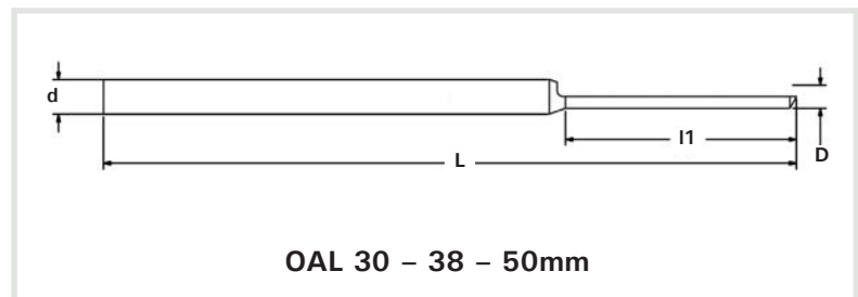
1100 Series Solid Carbide Half Round Gun Drills- Drill Sizes 0.20 – 3.00mm
