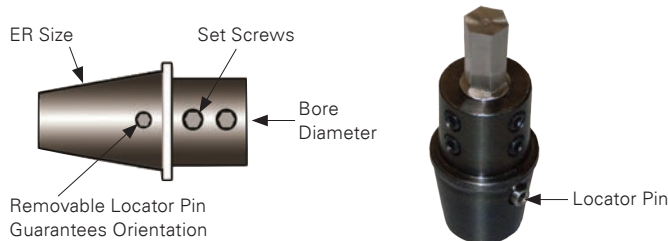
Punch Broach / Boring Adapters & Nuts
