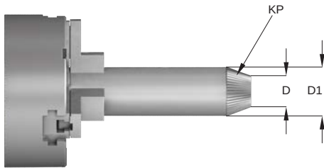
Figure 7 - Taper Knurling
