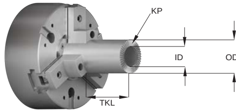
Figure 6 - Face Knurling
